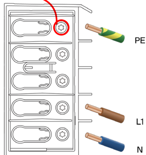
TN/TT 1-phase (230V)
