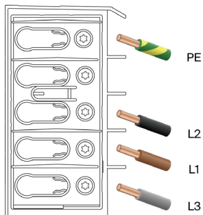
IT/TT 3-phase (3 x 230V)
